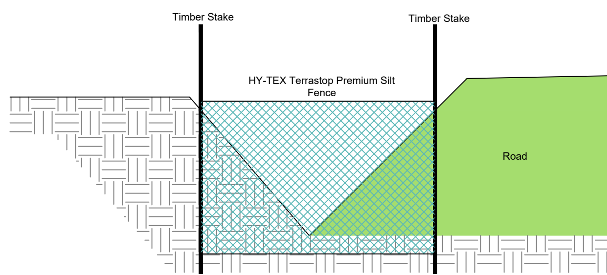
Sediment Fence Check Dam Detail
