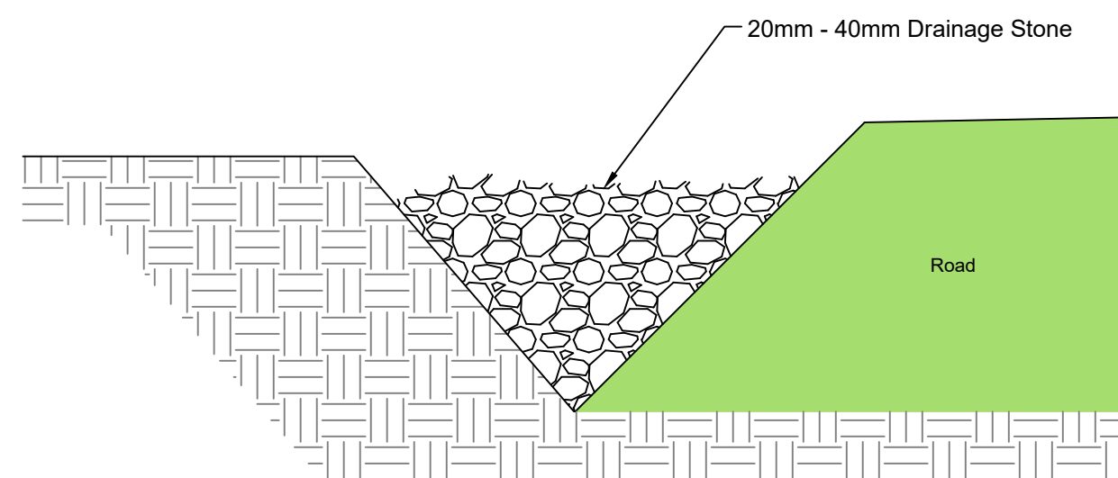
Stone Check Dam Detail
